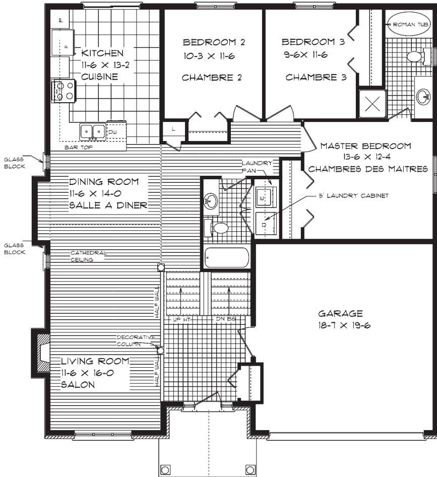
OPTIONAL TWO BATHROOM, 3 BEDROOM PLAN MAIN FLOOR PLAN PLANCHER PRINCIPAL
