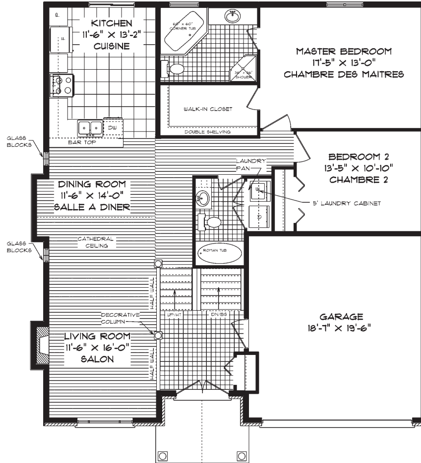
OPTIONAL TWO BATHROOM, 2 BEDROOM PLAN MAIN FLOOR PLAN PLANCHER PRINCIPAL
