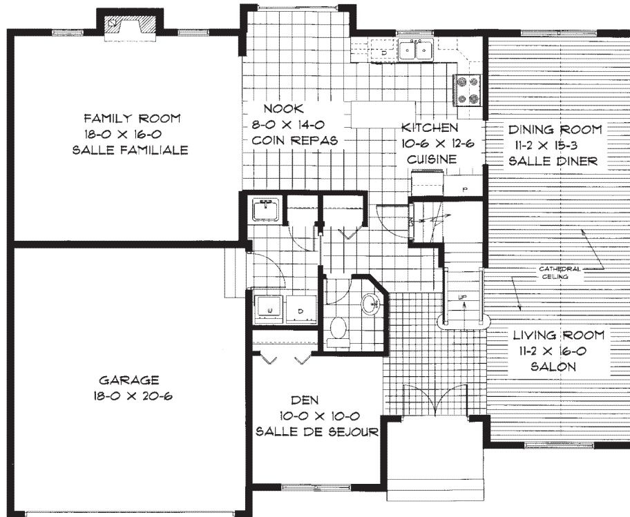
GROUND FLOOR PREMIER PLANCHER
