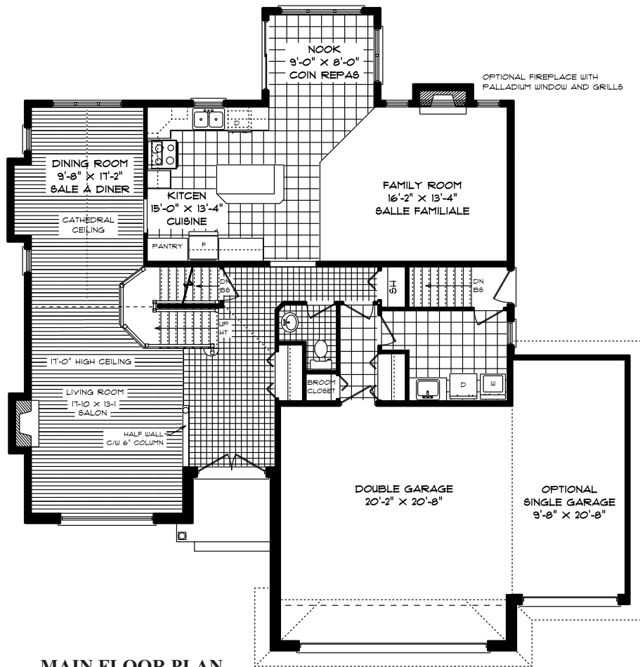
MAIN FLOOR PLAN PLANCHER PRINCIPAL
